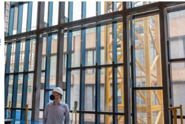
Where possible, exterior glass in the Peabody has been fritted to reduced the number of bird strikes.
